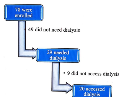
Figure 1: The Study Flow Chart
