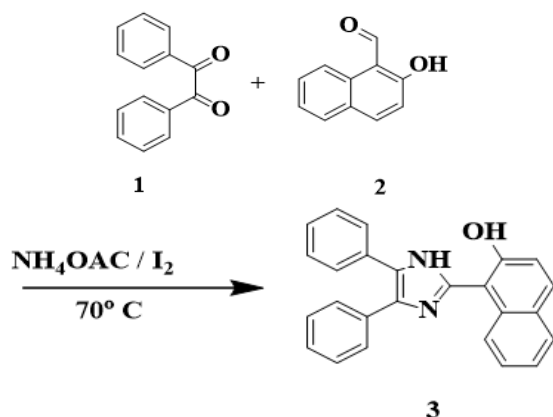
Scheme 1: Synthetic route for iodine assisted synthesis of 1-(4,5-diphenyl-1H-imidazol-2-yl)naphthalen-2-ol (3).
