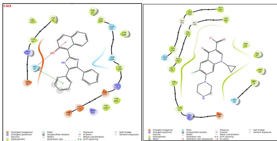
Figure 1: 2D docking poses / binding patterns with 3AC
