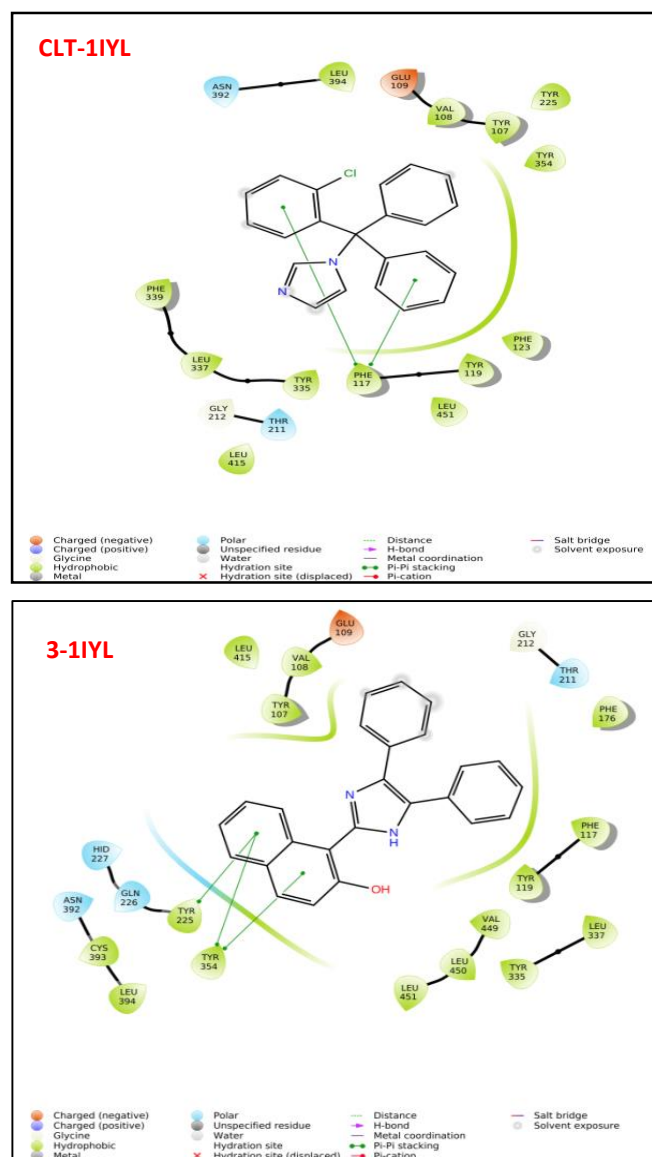
Figure 2: 2D docking poses / binding patterns with 1IYL
