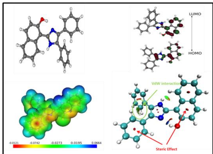
Figure 3: HOMO-LUMO energy gap of compound along with electrostatic potential diagram and RDG
