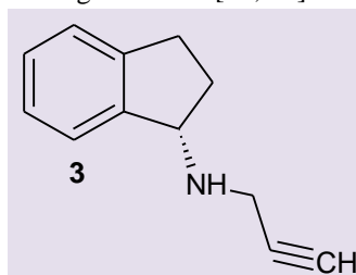
Figure 3: Structure of Rasagiline S -form
